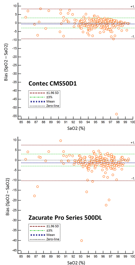
Figure 2 Bland-Altman plots of the bias compared with SaO 2 of two pulse oximeters with the lowest mean bias (Contec CMS50D1 −0.6 and Zacurate Pro series 500 DL −1.4). *Bland-Altman plots for each pulse oximeter to graphically display its bias (SpO 2 −SaO 2 ) to the reference standard (SaO 2 ). We added a zero-line and upper and lower limits of agreement ( \pm 1.96 SD). To visualise the accuracy standards required by the regulatory bodies, \pm 3\% lines are also displayed in the figures. *Bland-Altman plots of the other pulse oximeters can be found as a supplemental figure.
