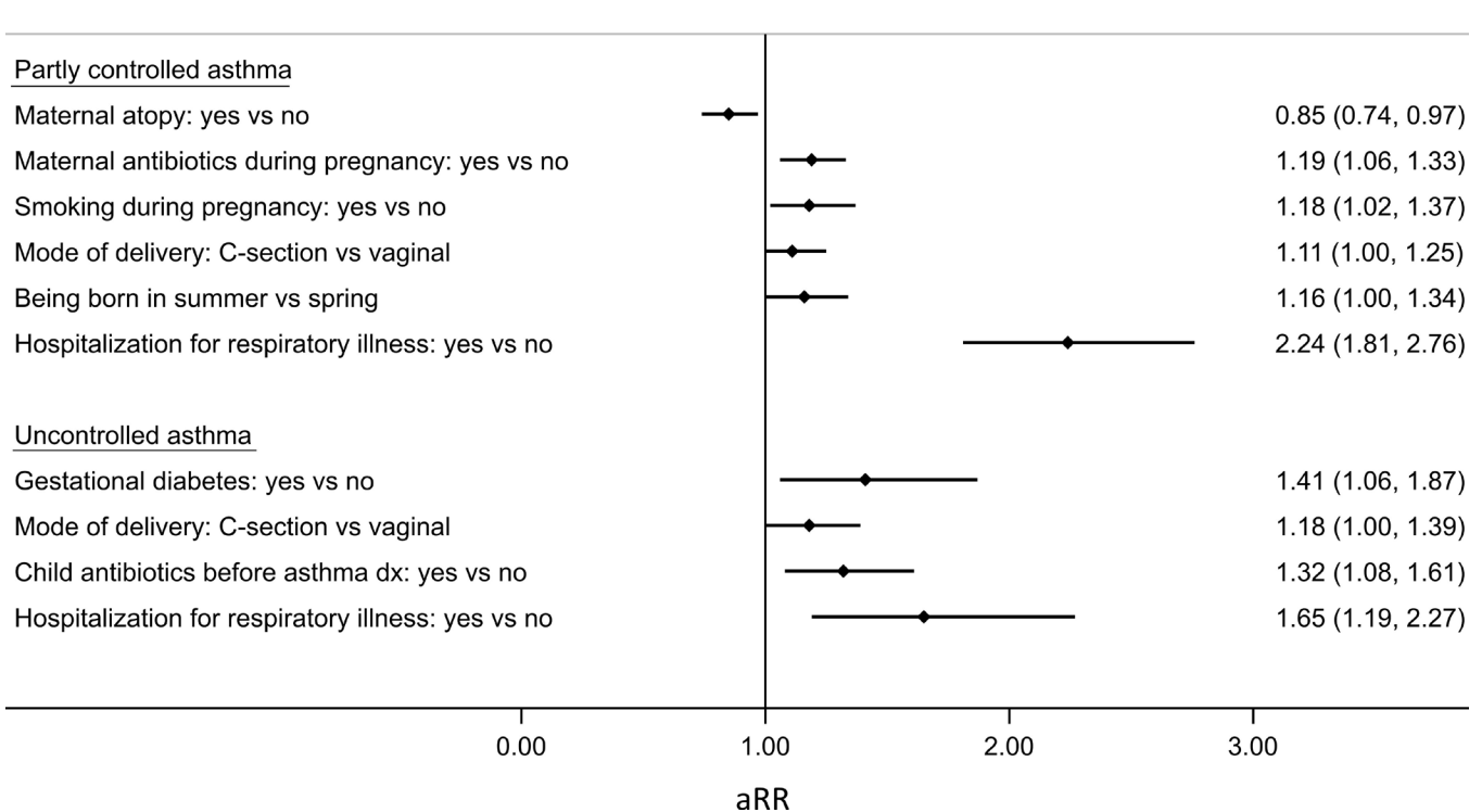
Figure 2 Relative risk of partly controlled (n=2629) and uncontrolled asthma (n=849) compared with controlled asthma (n=3728) assessed within the first 2 years of the initial diagnosis according to maternal and perinatal risk factors. The relative risk associated with each exposure and outcome is adjusted for all other exposures included in the figure, and covariates (child sex: male vs female, and maternal material socioeconomic status: low vs high). P value for model <0.0001, LR \chi^2 : 118.89.
