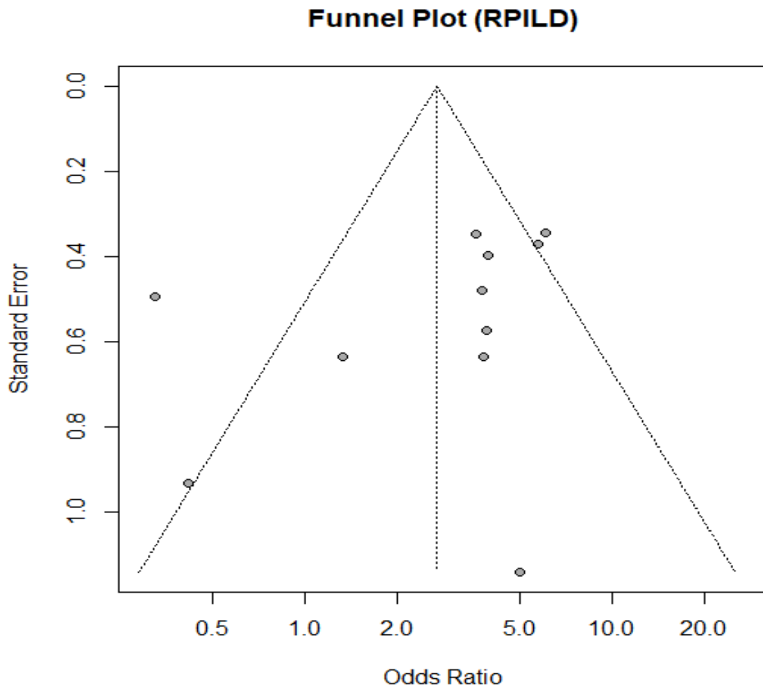
Supplementary Figure 2. Funnel plot of studies demonstrating the association between anti-Ro52 and RPILD
