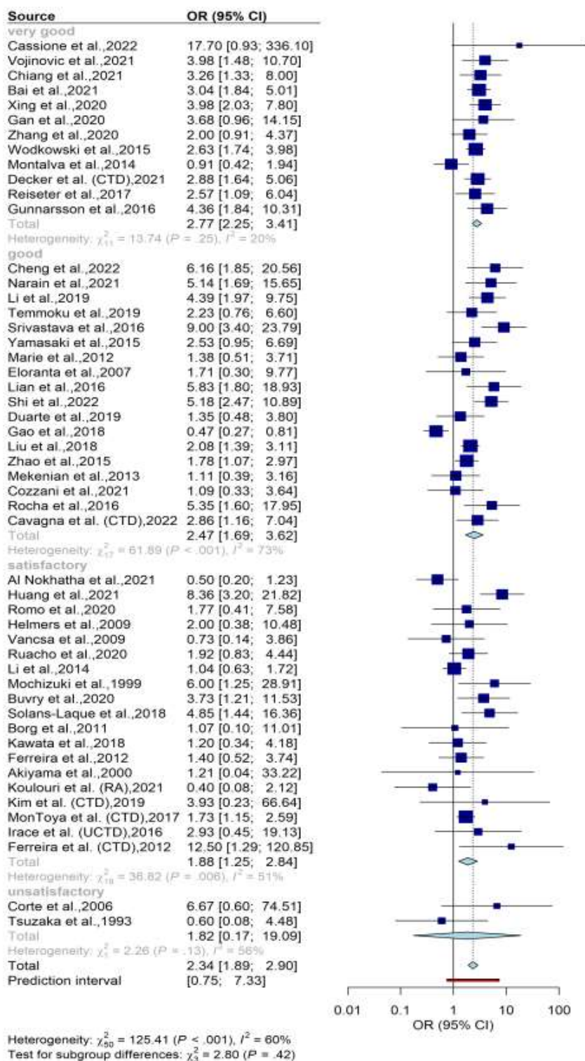
Supplementary Figure 3. Sensitivity analysis based on quality assessment of the studies.
