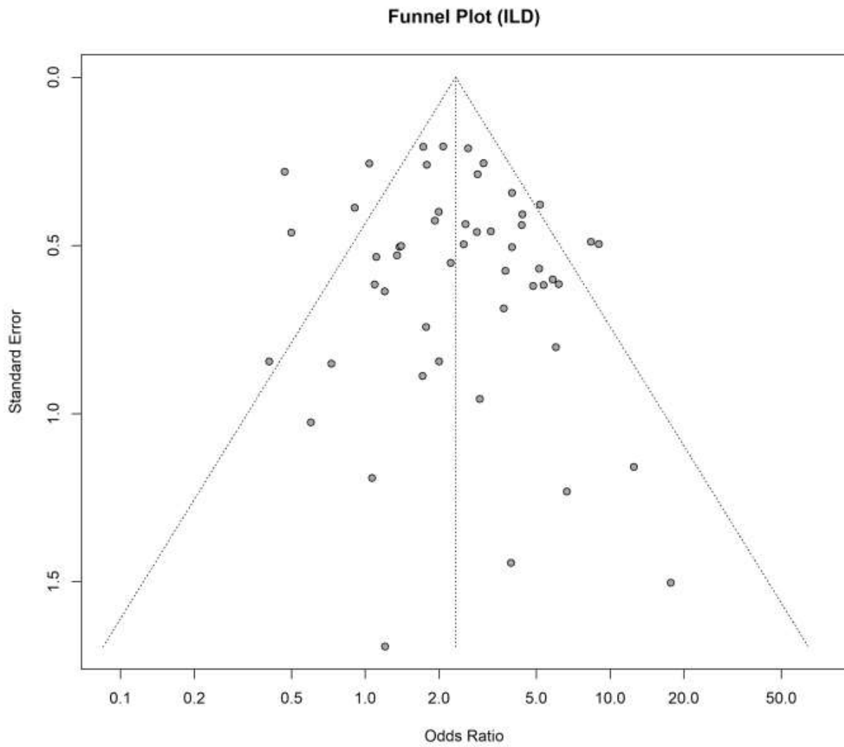
Supplementary Figure 1. Funnel plot of studies demonstrating the association between anti-Ro52 and ILD
